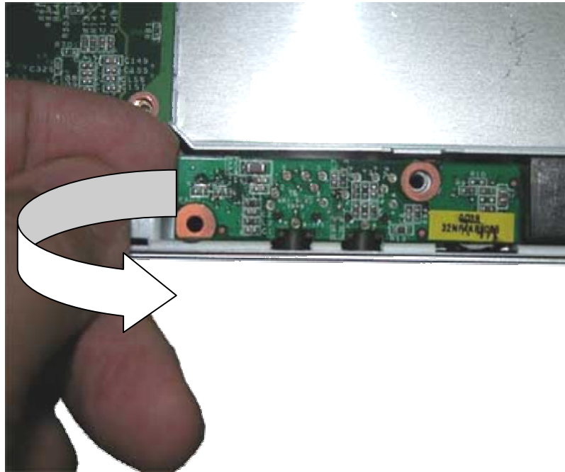
Fig. 30 Lifting up the audio board
